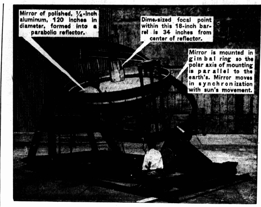
Mirror of polished, 1/4-inch aluminum, 120 inches in diameter, formed into a parabolic reflector. Dime-sized focal point within this 18-inch barrel is 34 inches from center of reflector.
