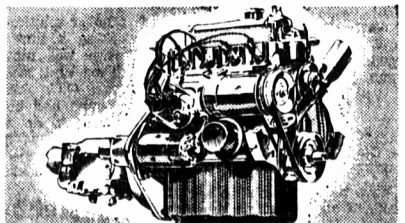
New Overhead Valve Engine was used in test car. The new 4-cylinder engine is a standard feature of all new Morris Minors. Engine has mixture control and throttle interlocked—gives faster starts, even in coldest weather.
