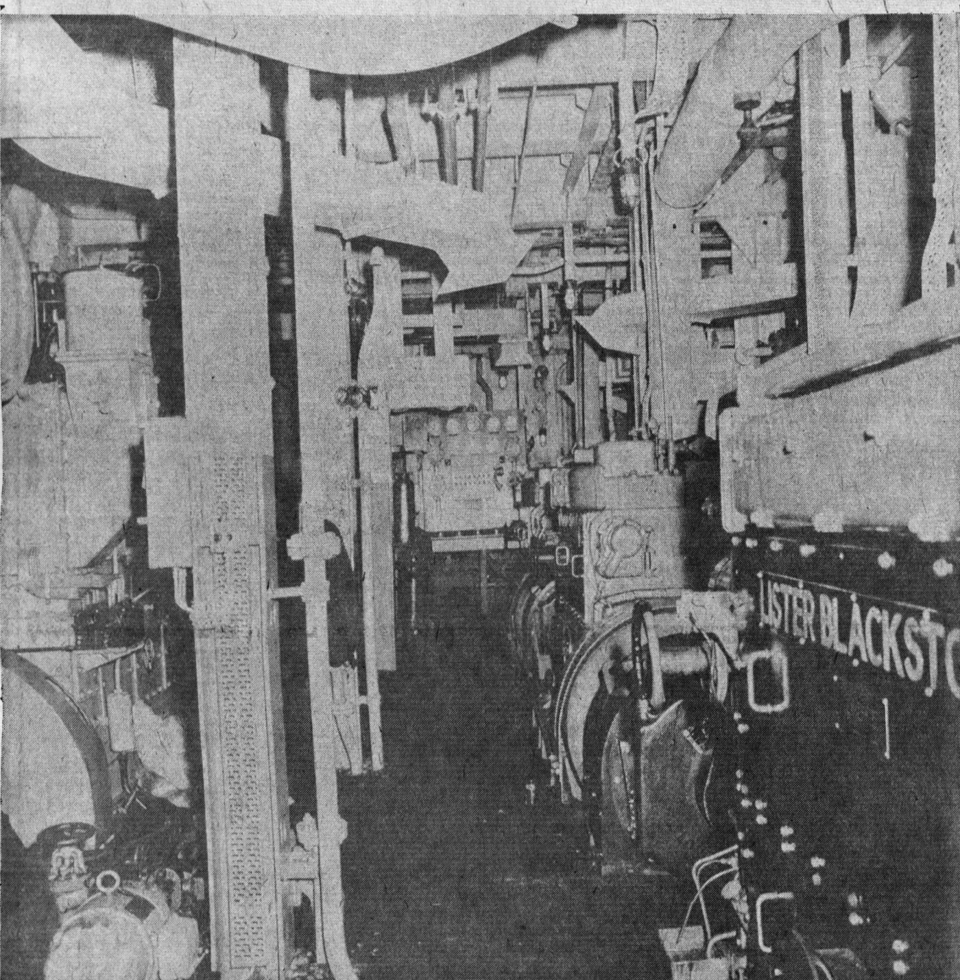
A VIEW of the Lord Selkirk's engine room showing main engines and auxiliary generators. Note engine room controls at centre. This panel is fitted with all gauges and instruments necessary for the full control of both engines.
