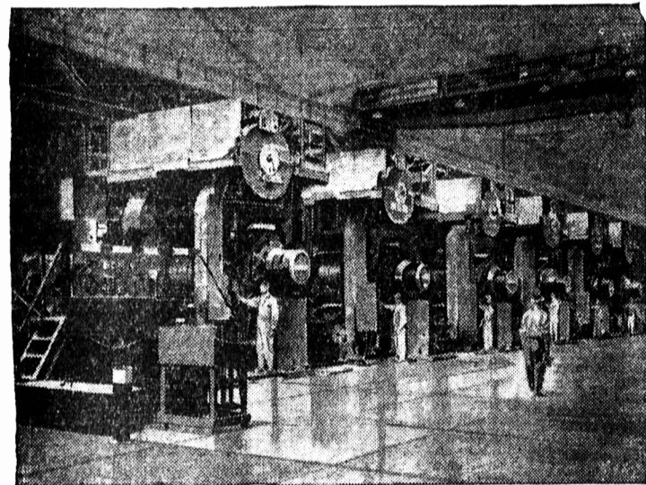
Stelco Continuous Hot Strip Mill produces steel sheets 49 inches wide at nearly 1800 ft. per minute!
