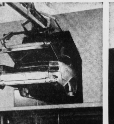
2. Tunnel. The car passes through an immense tunnel. Spray jets hammer every square inch of the car's surface to remove all impurities. On its way through, the car is Deep-dipped into six tanks containing rustproofing solutions.
