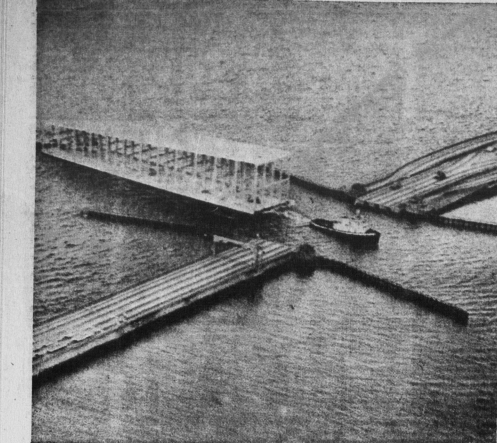
GANGWAY! The First Lake Washington Floating Bridge through the 360-foot pontoon, rising 53 feet above the water, was towed from Kenmore, where it was built, to the East Side of the Evergreen Point Bridge site. (AP Wirephoto)
