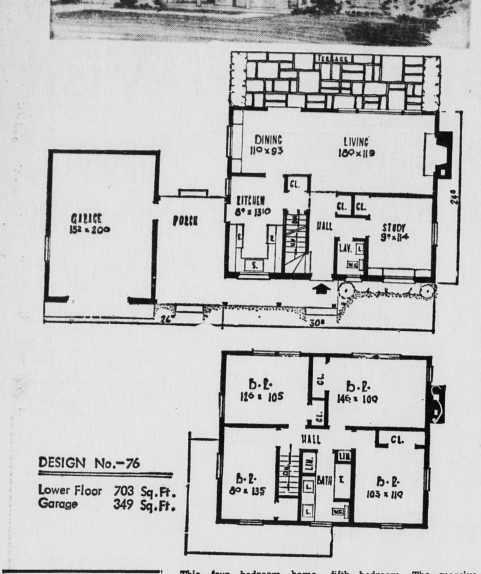
DESIGN No.-76 Lower Floor 703 Sq. Ft. Garage 349 Sq. Ft.
