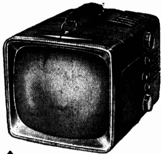
The Wayfarer. Model 14S707. Attractive 14 in. portable. Leather handle, telescoping V-type antenna, handy terminal connectors. 15 actual tubes. Red, gray or ivory finished metal cabinet. $189.95.
