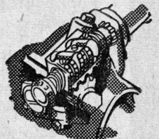
You get quick, easy response with Chevrolet's ball-bearing steering. Polished steel balls minimize friction — keep steering light but firm and positive.
