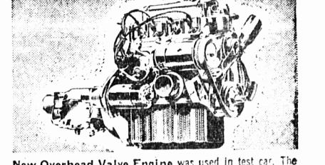
New Overhead Valve Engine was used in test car. The new 4 cylinder engine is a standard feature of all new Morris Minors. Engine has mixture control and throttle interlocked—gives faster starts, even in coldest weather.
