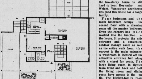
WHERE SPACE must go hand in hand with economy, the two-storey house is still hard to beat. Koyander & Wright, Vancouver architects, designed this house for a large family.
