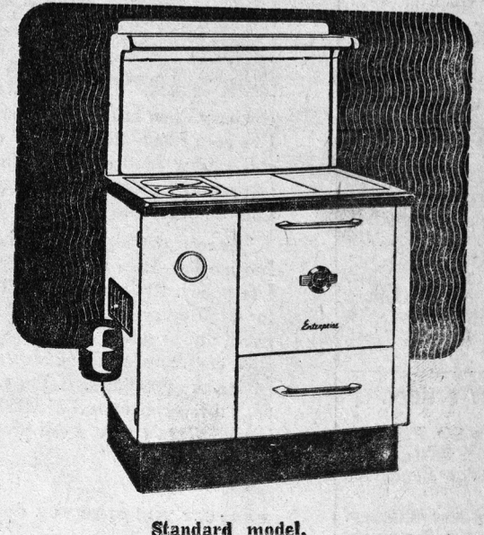
Standard model.
