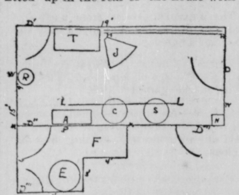
GROUND PLAN OF BUTTER ROOM.
