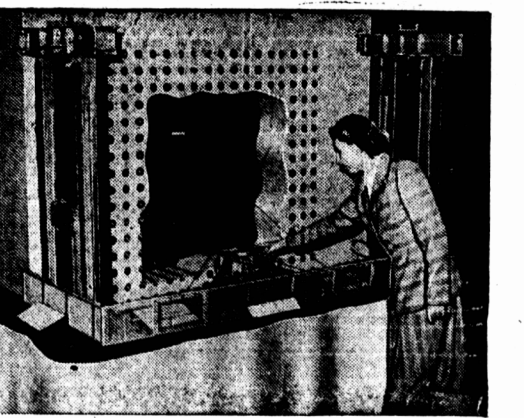
Miss Wildblood is here indicating rods used to control the power at which the pile runs.
