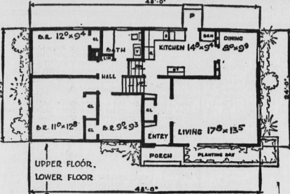
DESIGN No. 231 --- 1134 Sq. Ft. Gar. 240 " x 31 "
