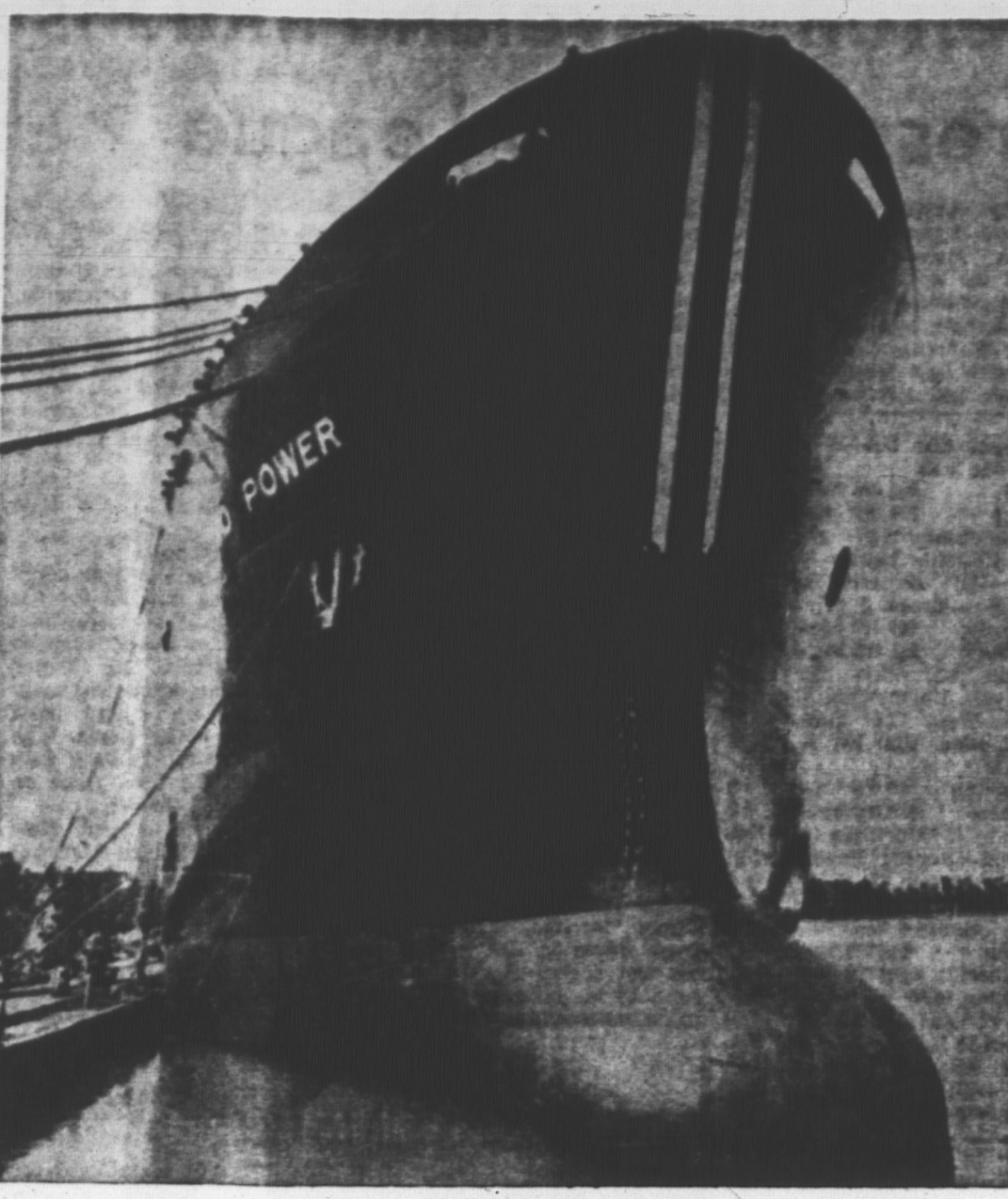
Headon view shows the unusual, bulbous, below-water bow of the SS Ontario Power, commissioned Saturday near St. Catharines, Ont., for the coal trade between Nova Scotia and Lake Ontario. The 710-foot, 22,500-ton capacity bulk carrier, is the largest ocean-going vessel ever built on the Great Lakes. The bow design makes her sea-keeping qualities and speed as efficient on the Seaway as the ocean. (CP Wirephoto).
