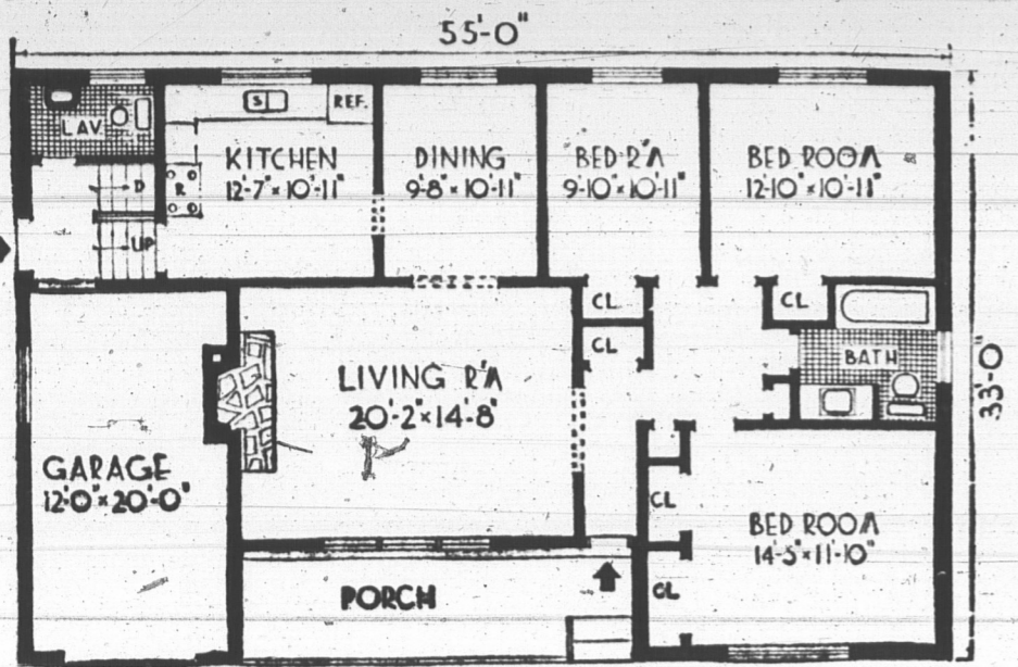
DESIGN CH-804 HOUSE-1450 SQ.FT. GARAGE-240 SQ.FT.
