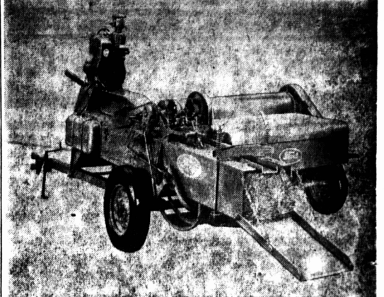
Ford Motor Company announces a new automatic twine tie baler, designed for one-man operation and employing sweep fork feed, unique in the lowest-priced baler field. The new four-bales-a-minute machine is the Ford 250, available in three models, engine driven with starter or without starter, and power take-off.
