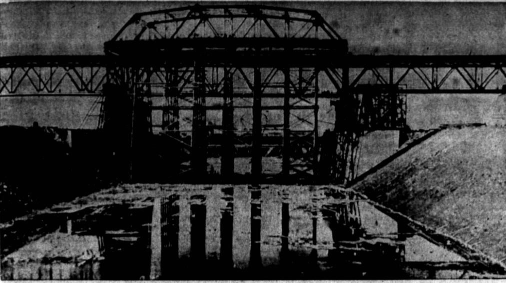
THIS PICTURE taken from the dry bed of seaway channel in St. Lawrence river at Montreal shows new 1,500-ton seaway-size span ready to slide into Jacques Cartier bridge.
