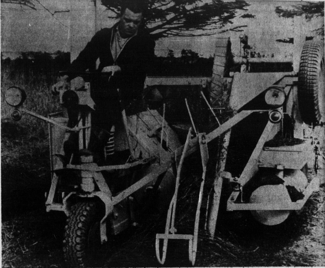
THIS BELGIAN-made binder is seen picking up the cured flax from the swath on the farm of Theo Foy, Augustine Cove. Operating the machine is Duane Mar-
