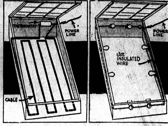
Either Heating Cable or Electric Lamps Will Heat a Hotbed.
