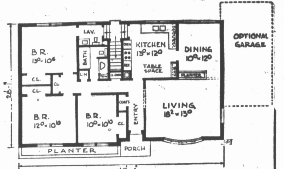
Design No. CH-1040 1362 Sq. Ft. Blueprints include complete details for building in BRICK or FRAME
