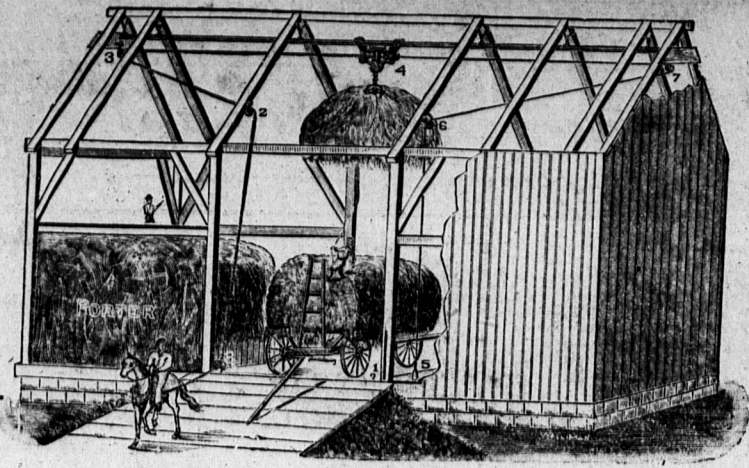
The above cut illustrates a "PORTER" (American) Haying Outfit, doing the work in a satisfactory manner.
