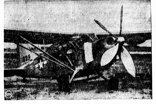
This Army Stinson L-5 is called the world's first "silent" airplane. Unveiled at Langley Field, Va., the plane's five-blade propeller is driven at 1000 RPM by an engine geared down to a ratio of 2.8 to one. It replaces a standard two-blade propeller driven directly by an engine operating at 2500 RPM. The reduction in speed, the Army says, is responsible for the reduction in noise.
