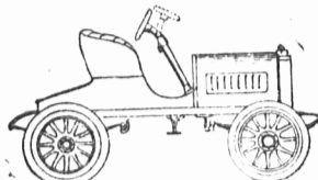
FLEXIBLE STEERING ROD FOR AUTOMOBILES.
