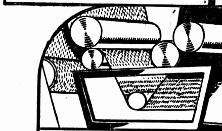
SAFTI-LOCK GUM-DIPPED CORD BODY. The long-staple cotton fibers of every cord are locked together for extra strength. These cords are then dipped in a special rubber solution for extra protection against blowouts.
