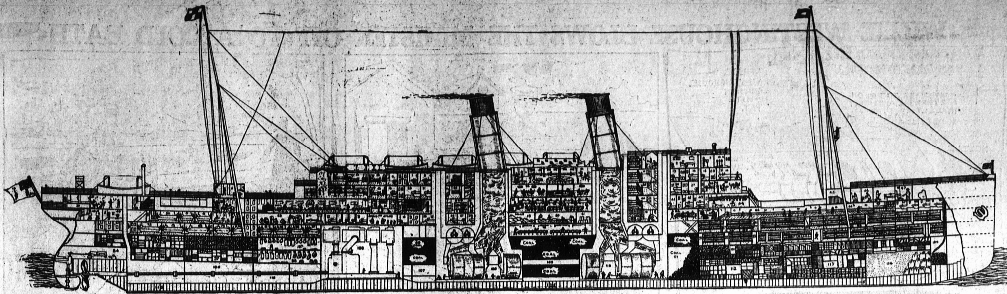
Canadian Pacific Railway Co's Twin-Screw Steamers "EMPRESS OF BRITAIN," and "EMPRESS OF IRELAND." Length 550 ft., Breadth 85 ft., Gross Tonnage 14,500.
