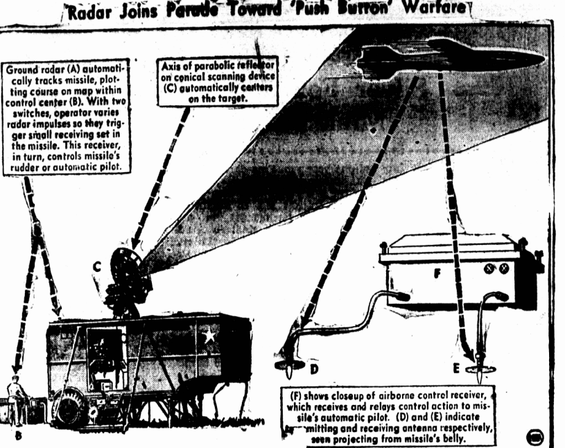
Diagram above, prepared from USAAF Air Materiel Command data, shows how ground radar now can control course of winged "buzz" bombs or rockets, as recently demonstrated at Wright Field, Ohio. Size of missile in sketch is exaggerated—actually it would be far out of sight of control operator. In this, radar control differs from that employing conventional radio waves, as with latter it is necessary for operators to see object being controlled. Research is now under way toward new systems capable of guiding several missiles at extreme altitudes and ranges.
