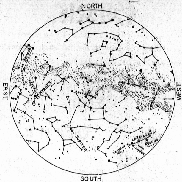
MAP OF THE DECEMBER HEAVENS. (Hold Back of Map to the Sky).
