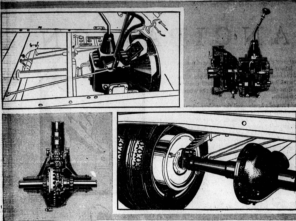
NEW SPIRAL BEVEL GEAR 3/4 FLOATING REAR AXLE Strength, reliability and long life
