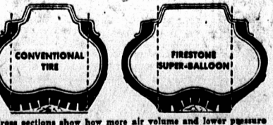
Cross sections show how more air volume and lower pressure permits greater flexing action when Firestone Super-Balloons go over bumps and rough roads.
