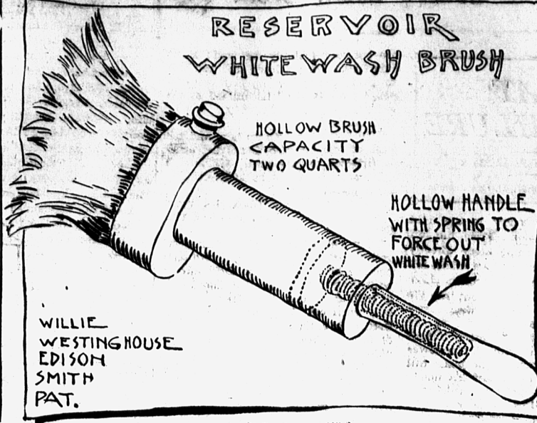
As he had about half a mile of them to do, I made him a brush like this diagram.
