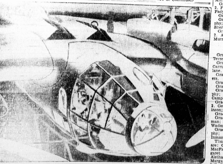
Experts of the R.A.F. take a view from the nose of a giant Heinkel III captured after an air raid on England. The machine crashed, very little damage and thus many of the secrets could be studied. Through the open trap under the fuselage the bombs which the Nazi airmen scattered indiscriminately, were dropped. This picture was taken from the London Daily Telegraph and arrived in Canada on the flying boat Clyde.
