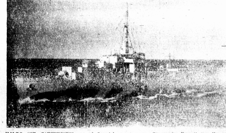
H.M.C.S. "ST. CATHERINES" one of Canada's recent destroyers, commanded by Lt.-Comdr. William P. Moffat, RCNVR of Montreal, was the first to see the U-boat and the first to score a hit after the sub was forced to the surface by depth charge attacks. (RCN Photo)
