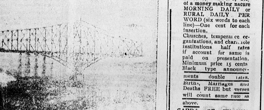
QUEBEC BRIDGE--SOUTHERN EXTENSION. It was the southern extension of the bridge which collapsed, and this was rapidly nearing the zenith of the immense steel arch which was to span the river. For eight hundred feet from the shore the massive structure reared its arch, with no supports but the piers from the shore, and one pier stood in the river, while the outward extremity was 180 feet above the water.
