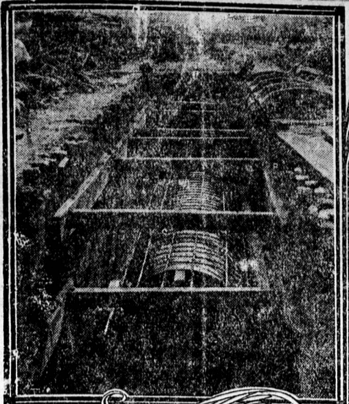
A Five Foot Outfall Sewer of Iron Pipe, Rod Be-en forced and Concrete Packed
