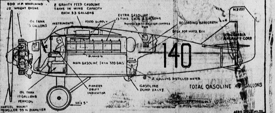
ABOVE is a diagram picture of the Columbia, the plane which carried Chamberlin and Levine successfully on their non-stop flight from the United States to Germany.
