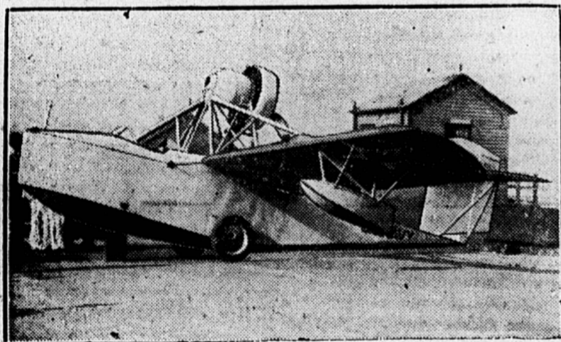
Here is a tiny monoplane-type flying boat constructed so that it can be folded up in three minutes and dropped into an eight-foot torpedo tube. One hundred and ten horsepower, it reaches a speed of 100 miles an hour. The hull, which is single-seated, is made of duralumin.—Associated Press Photo.
