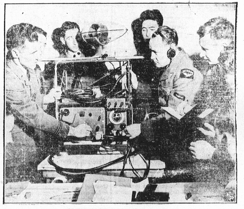
LEARNING TO PLOT SHORT ROUTES TO REICH. A group of students of the Commonwealth Air Training Plan surround a radio direction-finding device. Equipment of this kind is installed in all of Great Britain's bombing craft.
