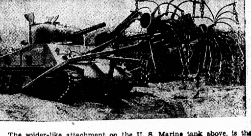
The spider-like attachment on the U. S. Marine tank above, is the "Sea Bee" answer to the peril of enemy-sown mines. Tubular hubs, from which chain-tipped flails hang, revolve rapidly, whirling the flails as they lash the ground, detonating contact mines which may be in the tank's path. They also set up an electrical field which explodes magnetic mines.
