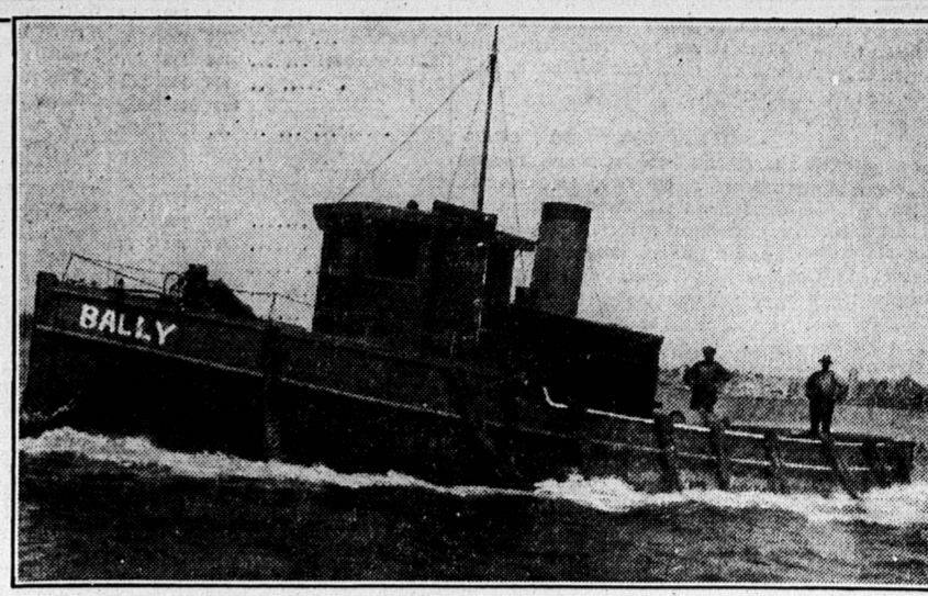
Tug "BALLY" Powered with Fairbanks-Morse 75 h.p. Marine Diesel Engine. Built from plans prepared by Fairbanks-Morse Engineers.
